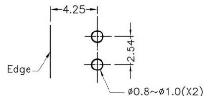
MOUNTING HOLES
