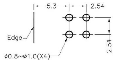
MOUNTING HOLE
