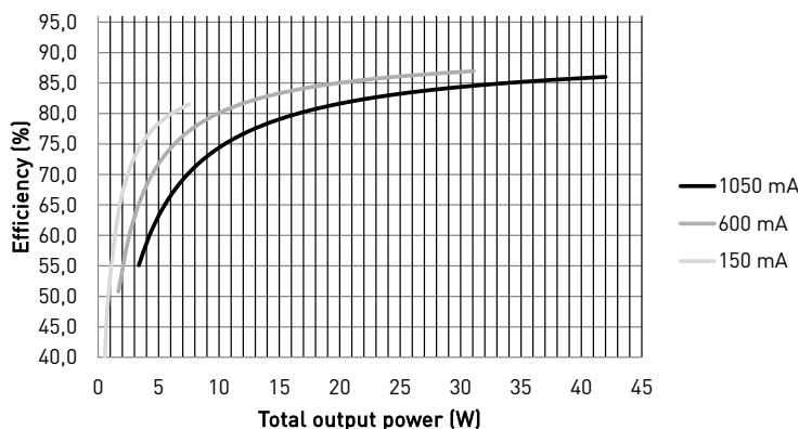
Typical efficiency
