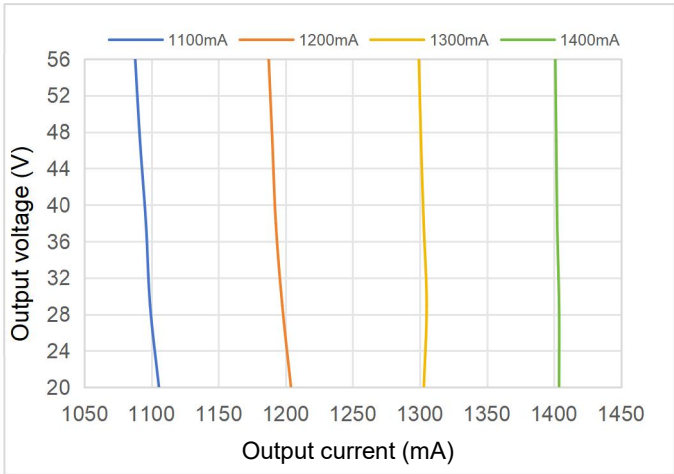
Operating Window
