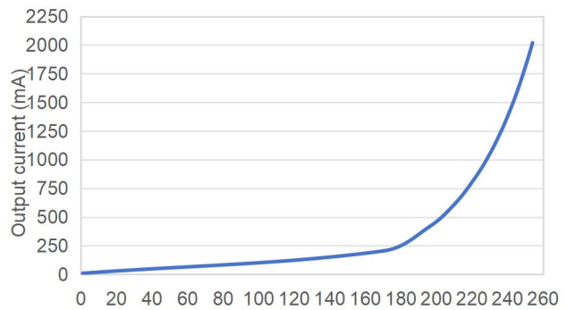
Logarithmic dimming
