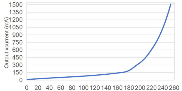
Logarithmic dimming
