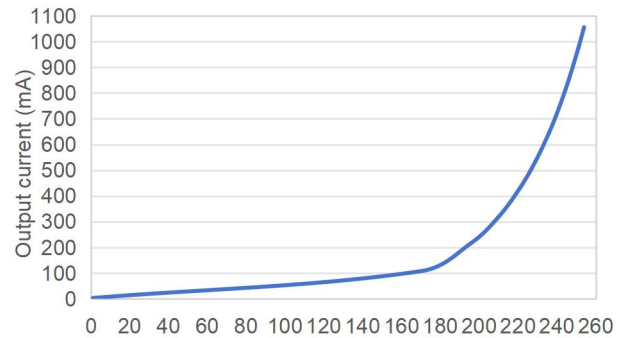
Logarithmic dimming
