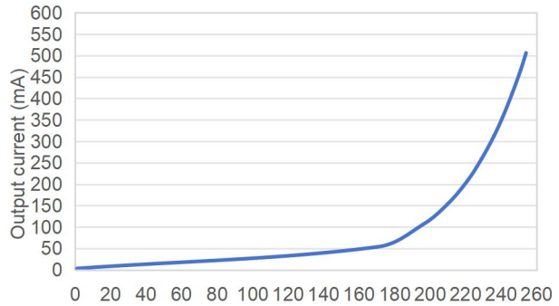
Logarithmic dimming
