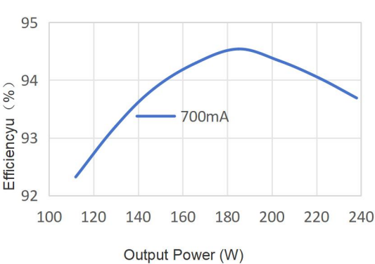
Typical Efficiency vs Load
