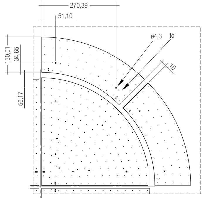
CLE Quadrant 541mm 1000lm ADV4
