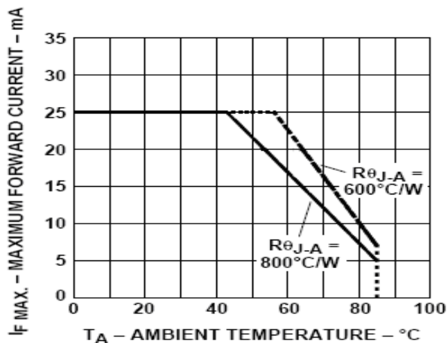
Figure 6: Derating Curve
