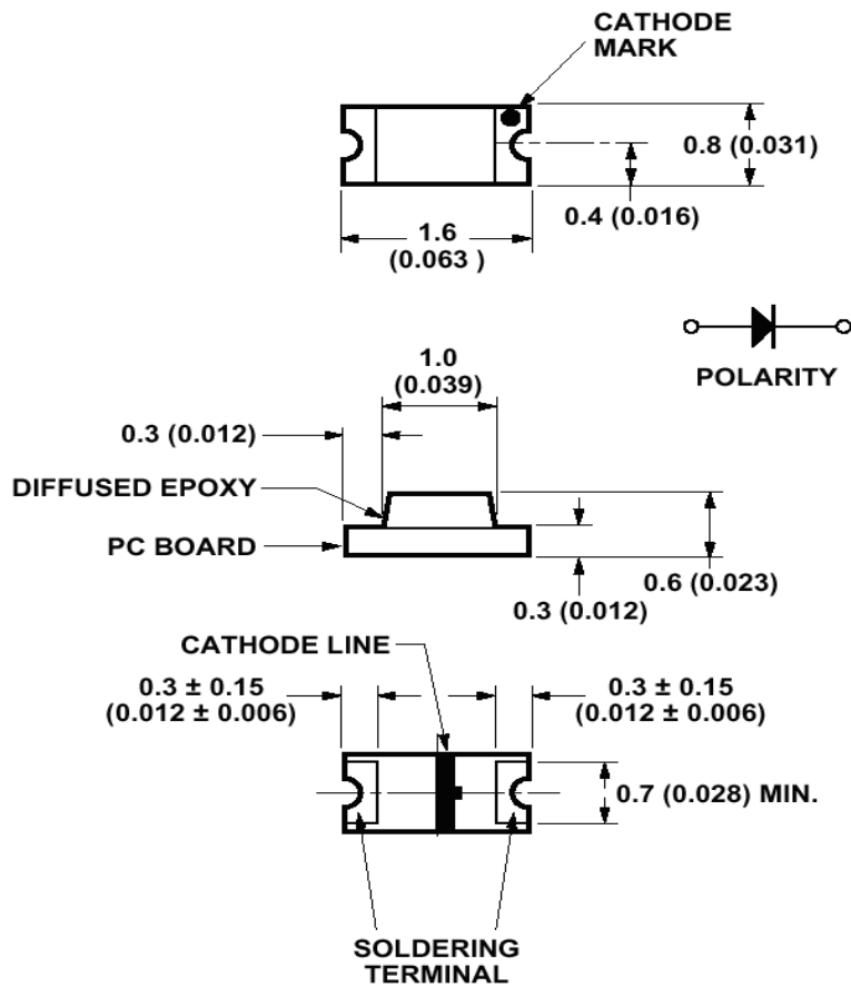
Figure 1: Package Dimensions
