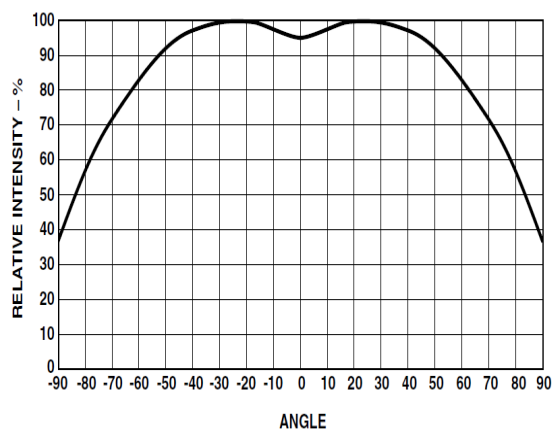
Figure 5: Radiation Pattern
