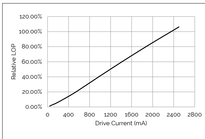
Figure 2: Relative LOP vs. Drive Current, T_c=25^\circ\text{C}
