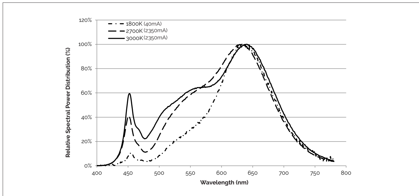
Figure 11: Typical Color Spectrum, T_c=25^\circ\text{C}
