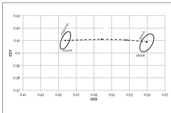
Figure 6: Color Shift vs. Forward Current 2700-1800K, T_c=25^\circ\text{C}
