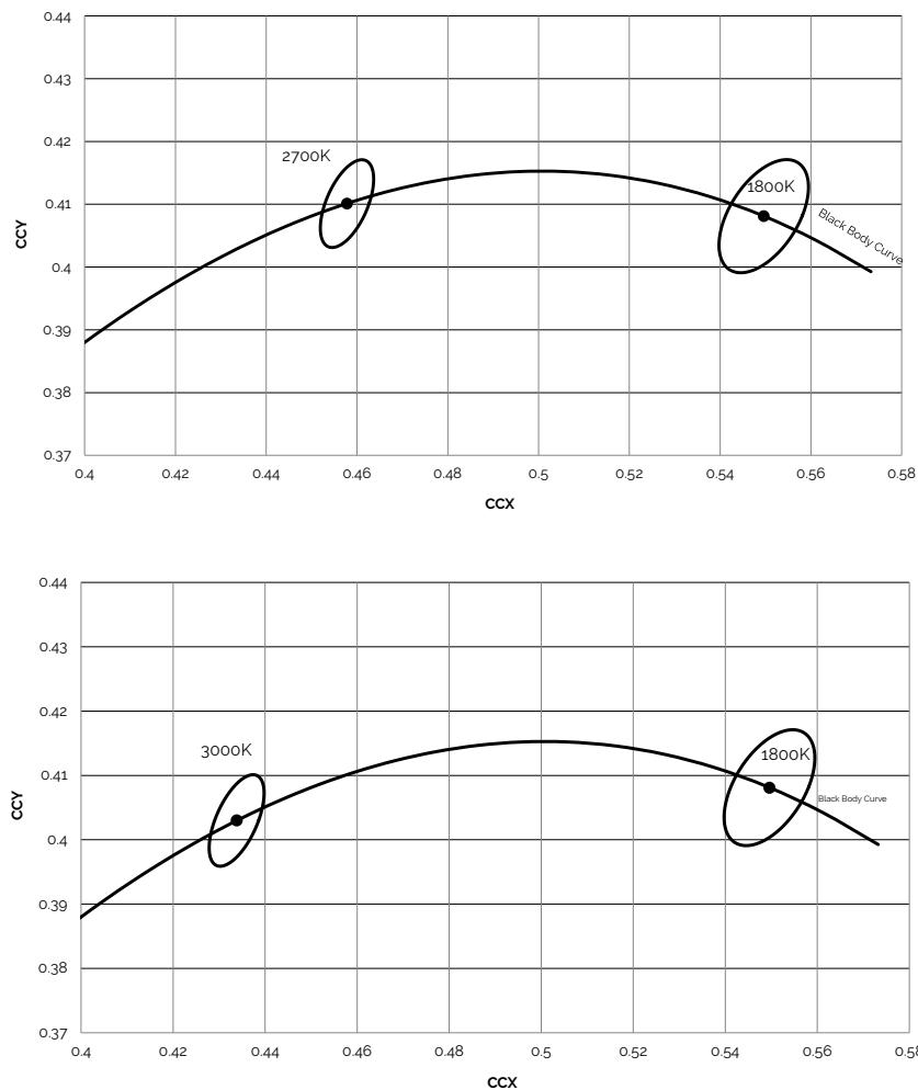
Figure 13: Graph of Warm White Test Bins in xy Color Space, T_c = 25^\circ\text{C}
