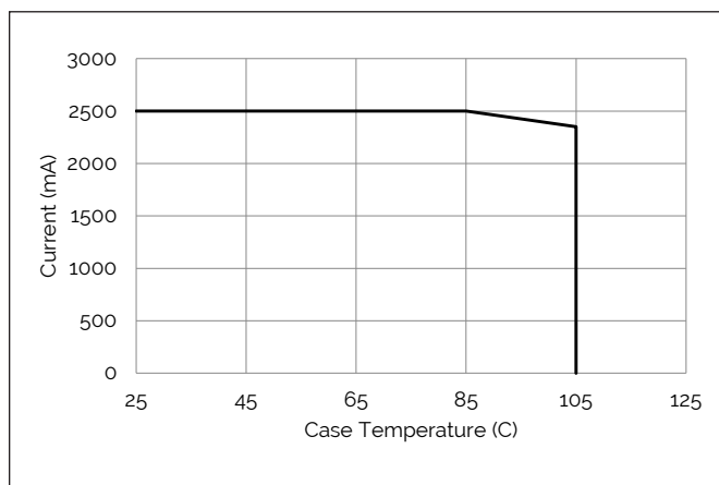
Figure 8: Derating Curve
