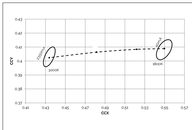
Figure 7: Color Shift vs. Forward Current 3000K-1800K, T_c=25^\circ\text{C}
