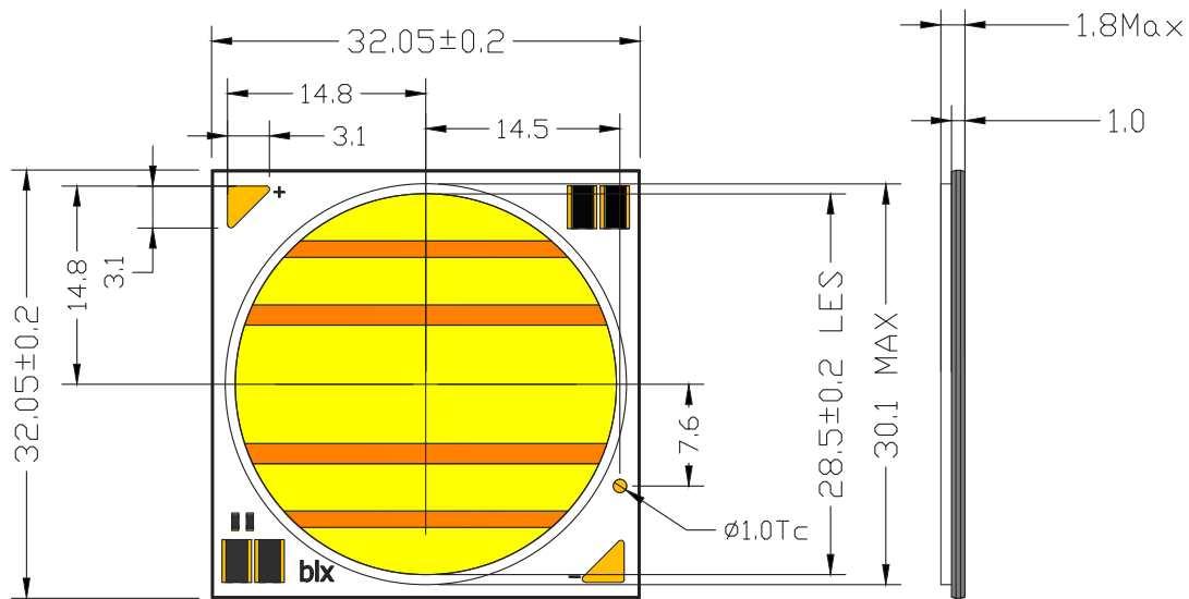
Figure 12: Mechanical Drawing
