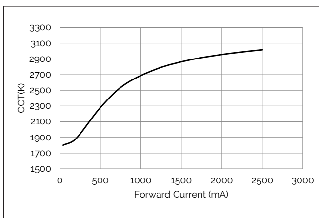
Figure 4: CCT vs. Forward Current, T_c=25^\circ\text{C}
