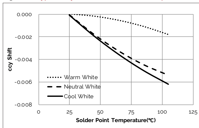
Figure 11: Typical ccy Shift vs. Solder Point Temperature 2,3,4,5
