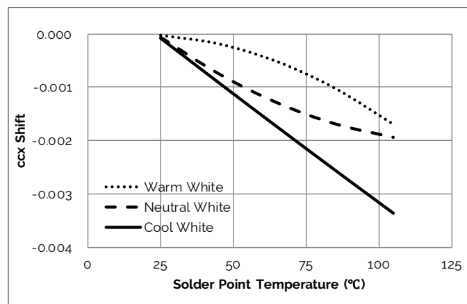
Figure 10: Typical ccx Shift vs. Solder Point Temperature 2,3,4,5
