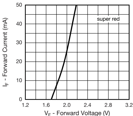
Fig. 2 - Forward Current vs. Forward Voltage (super red)
