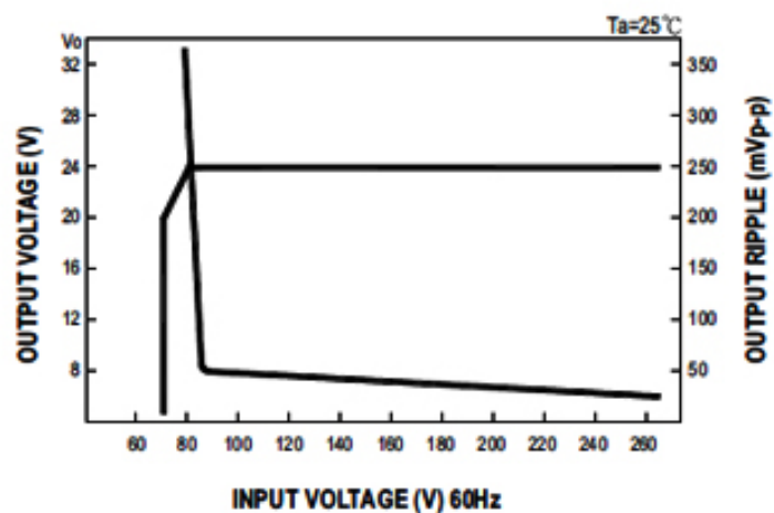
■ Static Characteristics (24V)
