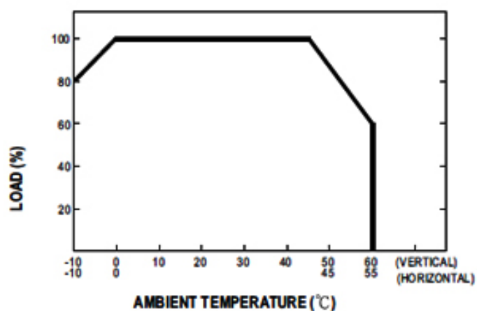
Derating Curve
